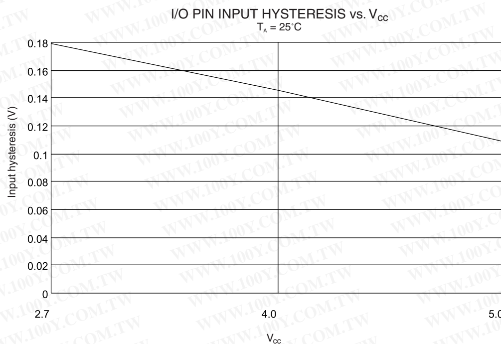
Figure 94. I/O Pin Input Hysteresis vs. V_{CC}
