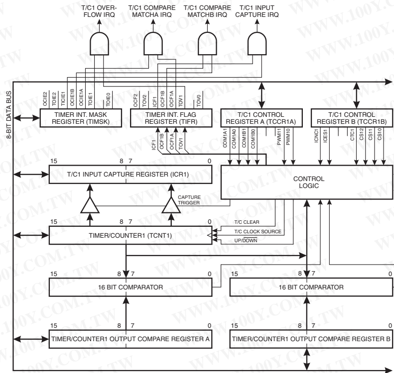
Figure 31. Timer/Counter1 Block Diagram
