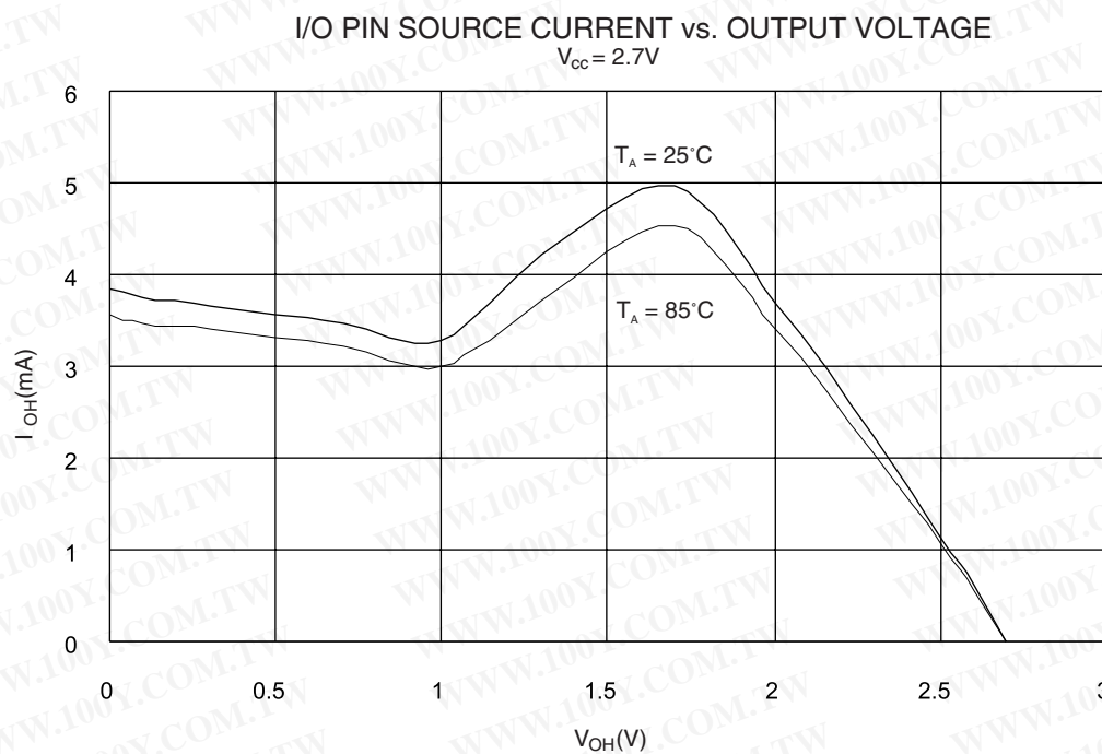
Figure 92. I/O Pin Source Current vs. Output Voltage
