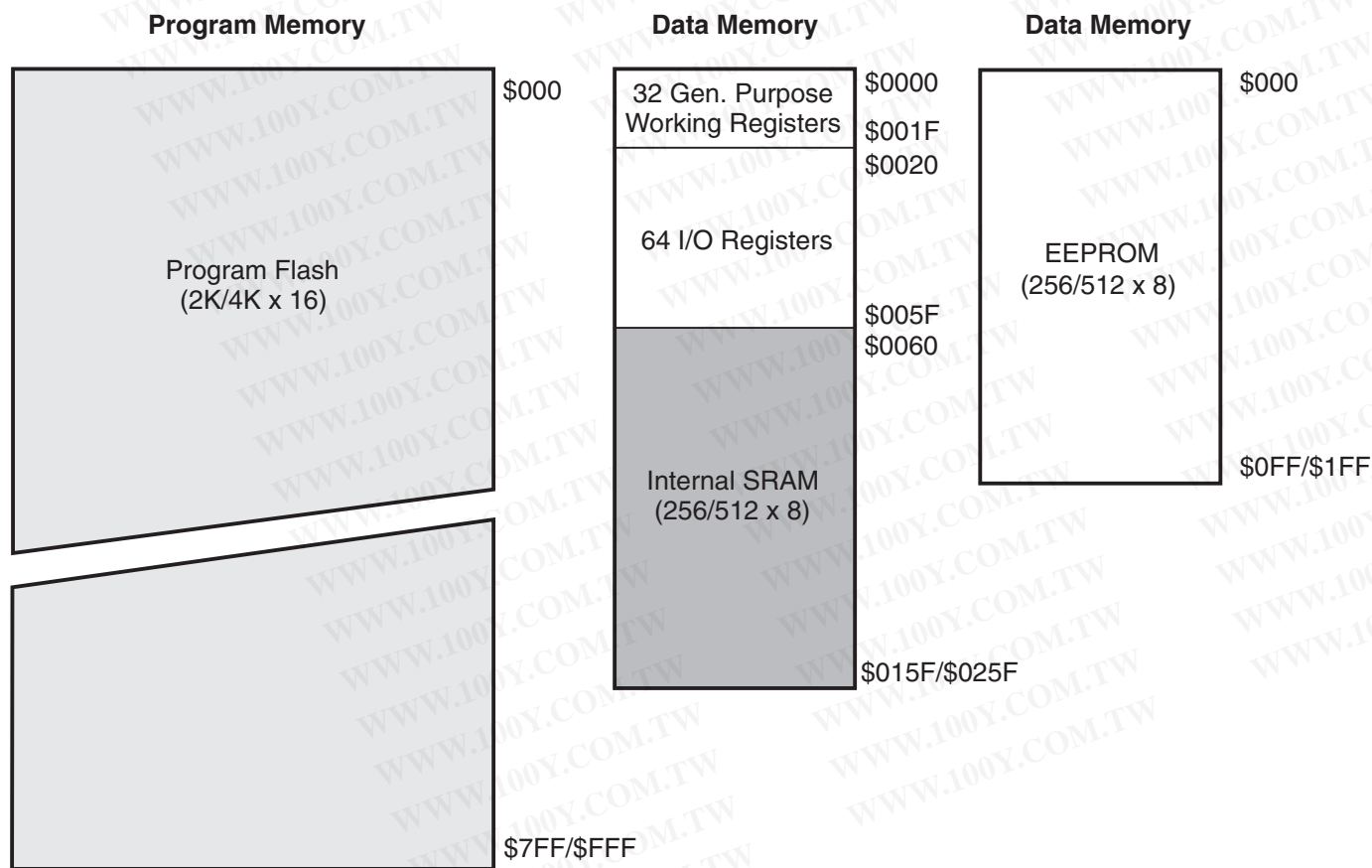
Figure 5. Memory Maps
