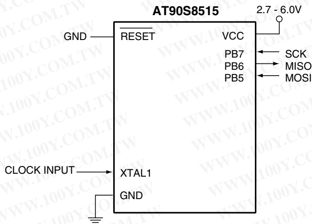
Figure 64. Serial Programming and Verify
