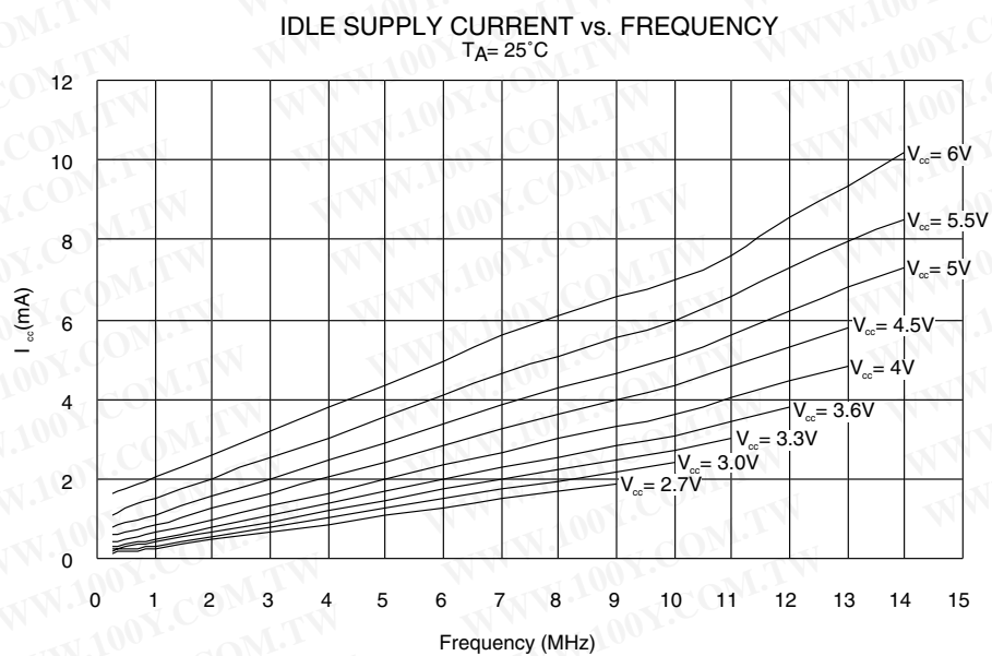
Figure 71. Idle Supply Current vs. Frequency
