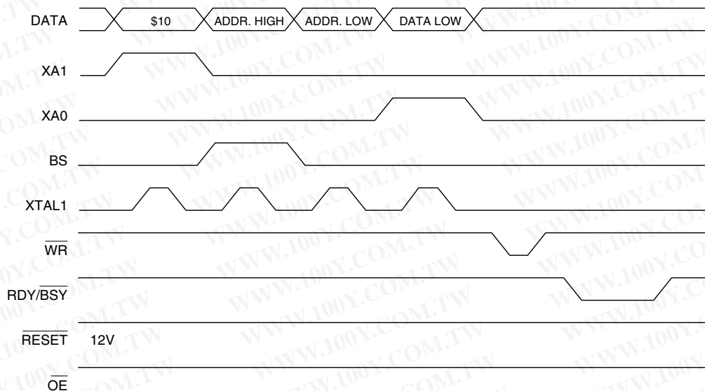
Figure 61. Programming the Flash Waveforms
