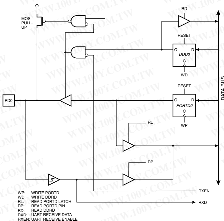
Figure 53. Port D Schematic Diagram (Pin PD0)
