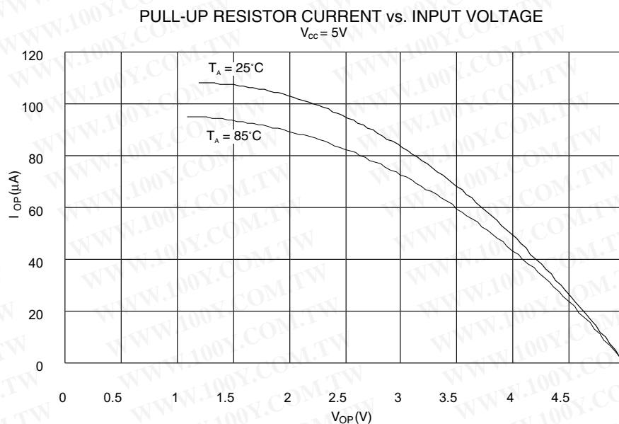
Figure 81. Pull-up Resistor Current vs. Input Voltage
