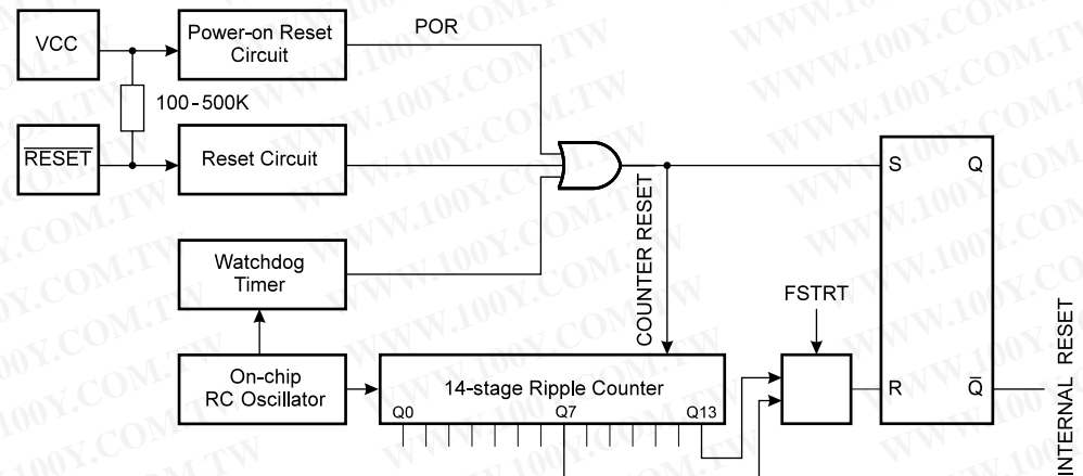
Figure 23. Reset Logic
