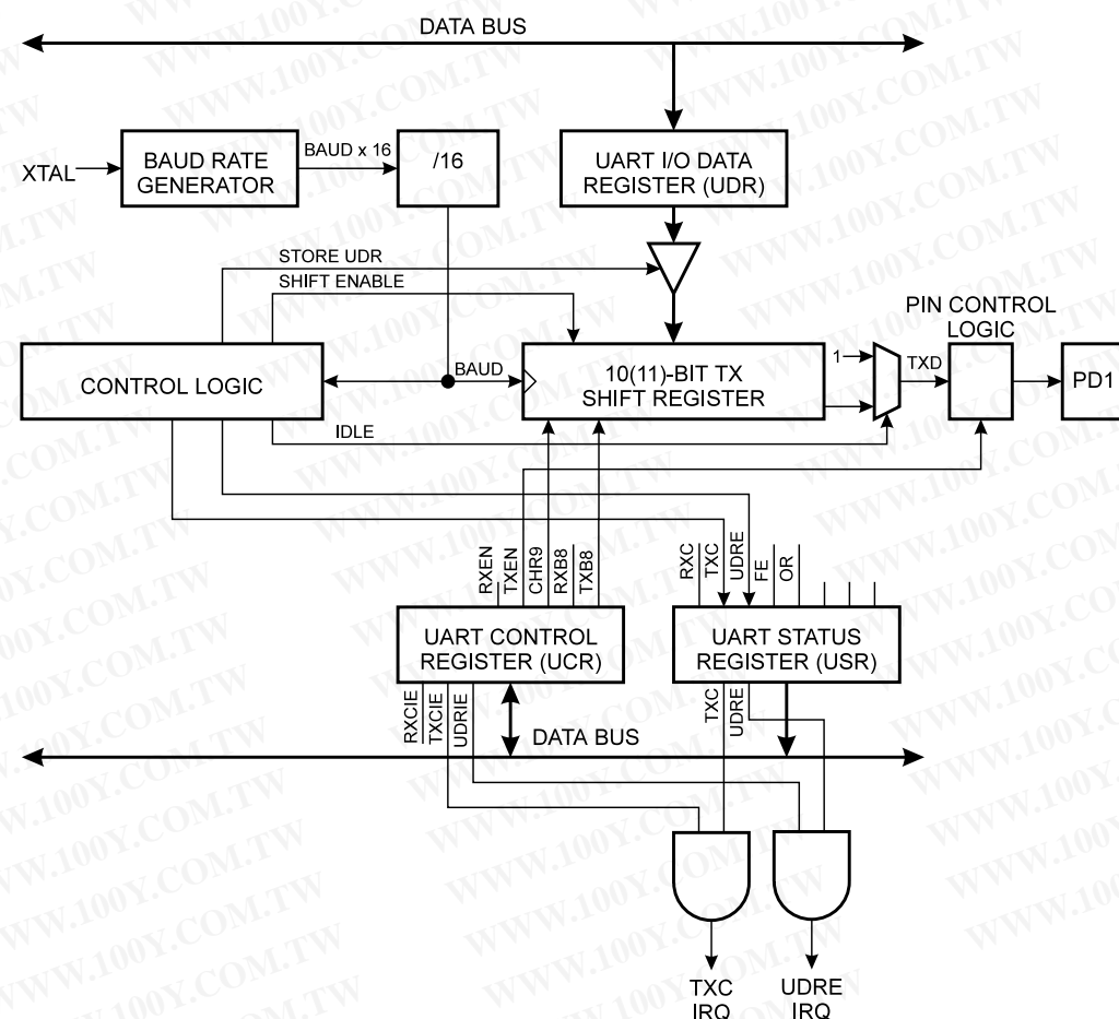
Figure 38. UART Transmitter
