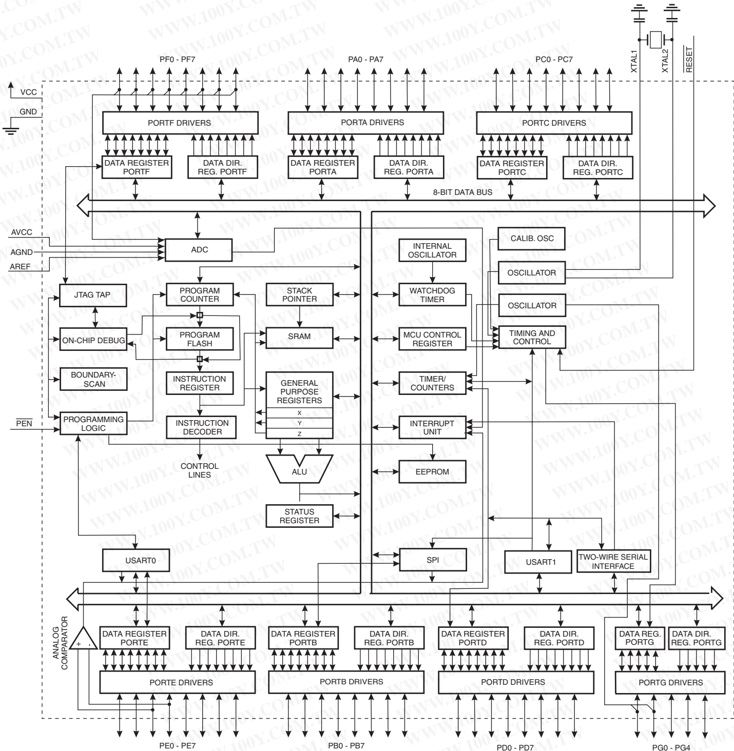
Figure 2. Block Diagram
