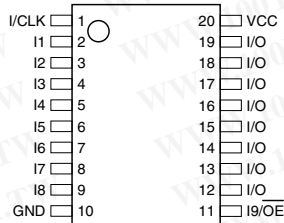
Figure 2-1. TSSOP
