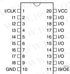
Figure 2-2. DIP/SOIC
