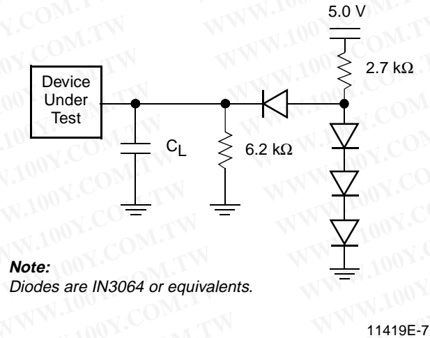
Figure 3. Test Setup
