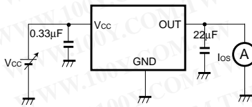
Fig. 5 Measurement circuit for output short-circuit current
