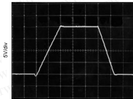
LARGE-SIGNAL STEP RESPONSE G = 1 , C_L = 300pF
