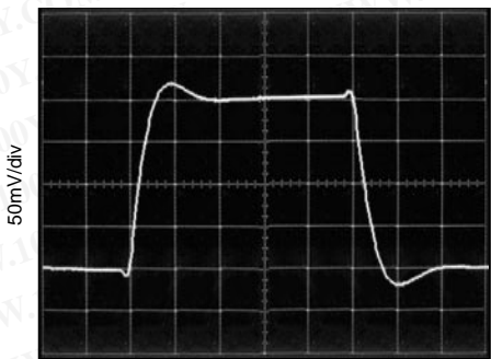
SMALL-SIGNAL STEP RESPONSE G = 1 , C_L = 300pF
