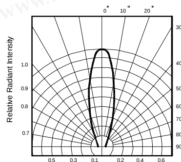
FIG.6 Radiant Diagram
