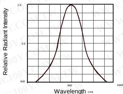
Fig.1 Spectral Distribution
