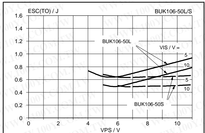
Fig.20. Typical overload protection energy, T_j = 25^\circ C E_{SC(TO)} = f(V_{PS}); conditions: V_{DS} = 13 V, parameter V_{IS}
