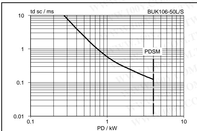
Fig.18. Typical overload protection characteristics. t_{dsc} = f(P_{DS}); conditions: V_{PS} \geq V_{PSP}; V_{IS} \geq 5 V
