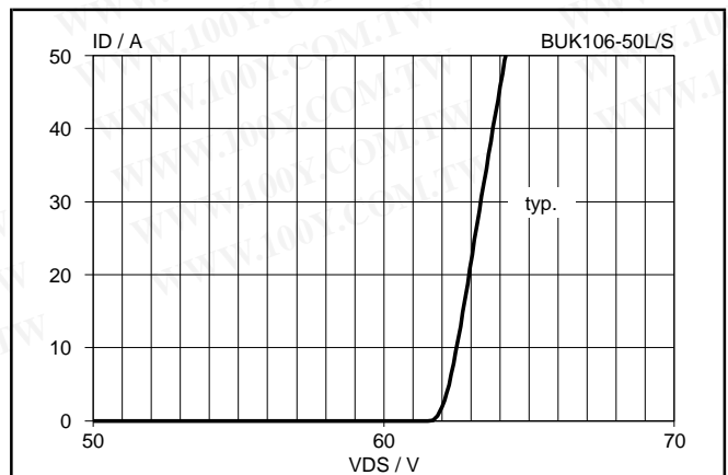
Fig.21. Typical clamping characteristics, 25^\circ C . I_D = f(V_{DS}); conditions: R_{IS} = 100 \Omega; t_p \leq 50 \mu s
