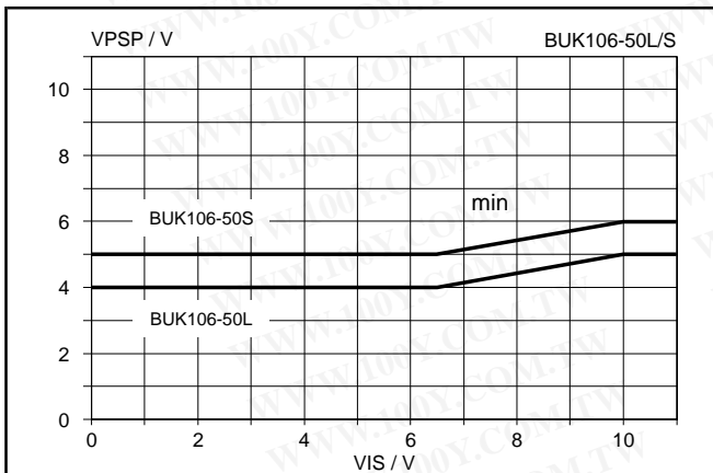
Fig.17. Minimum protection supply voltage for SC load protection. V_{PSP} = f(V_{IS}); T_{mb} \geq 25^\circ C
