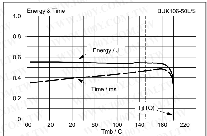
Fig.19. Typical overload protection characteristics. Conditions: V_{DD} = 13 V; V_{PS} = V_{PSN}; V_{IS} = 8 V; SC load
