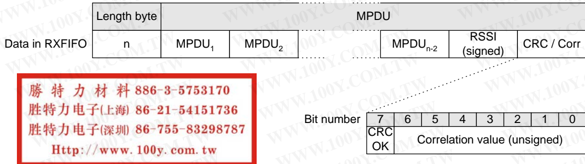
Figure 20. Data in RXFIFO when MDMCTRL0.AUTOCRC is set
