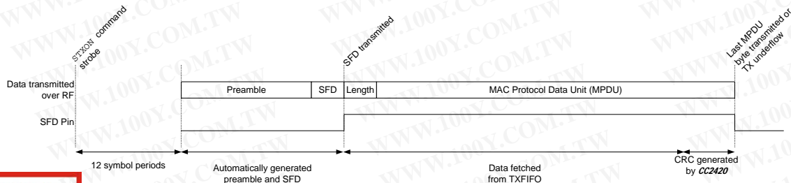
Figure 14. Pin activity example during transmit
