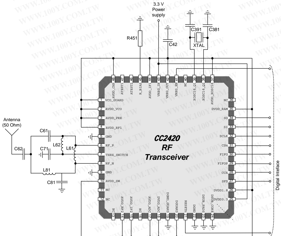
Figure 3. Typical application circuit with discrete balun for single-ended operation
