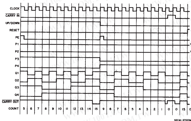
Fig. 16 — Timing diagram for CD4516B.
