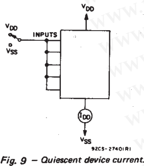
Fig. 9 - Quiescent device current.
