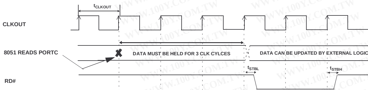
Figure 10-5. RD# Strobe Function when PORTC is Accessed by 8051
