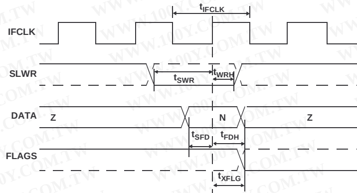
Figure 10-9. Slave FIFO Synchronous Write Timing Diagram [20]
