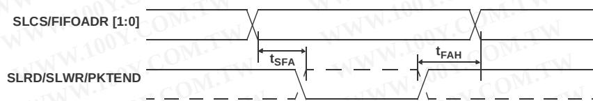
Figure 10-17. Slave FIFO Asynchronous Address Timing Diagram [20]
