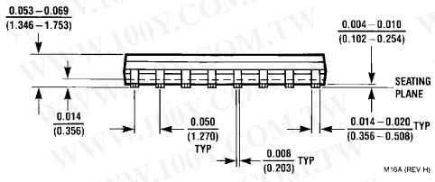
Molded Small Outline Package (SO) Order Numbers DAC0800LCM, or DAC0802LCM NS Package Number M16A
