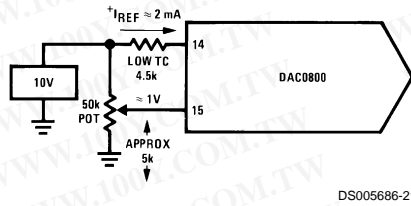
FIGURE 4. Recommended Full Scale Adjustment Circuit (Note 5)
