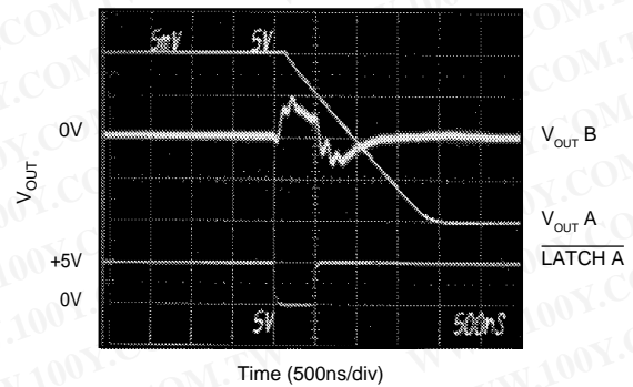
CROSSTALK (Bipolar Mode)
