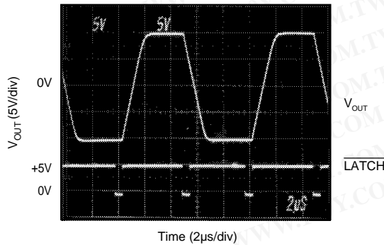
FULL-SCALE OUTPUT SWING BIPOLAR (20V Step)
