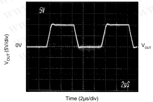
FULL-SCALE OUTPUT SWING UNIPOLAR (10V Step)
