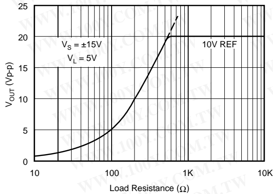
OUTPUT VOLTAGE SWING vs RESISTOR LOAD
