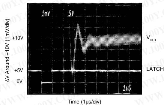
SETTLING TIME UNIPOLAR ( 0\text{V} to +10\text{V} Step)
