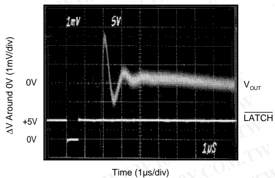
SETTLING TIME UNIPOLAR ( +10\text{V} to 0\text{V} STEP)
