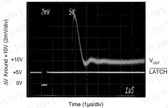
SETTLING TIME BIPOLAR ( -10\text{V} to +10\text{V} )
