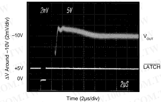
SETTLING TIME BIPOLAR ( +10\text{V} to -10\text{V} Step)
