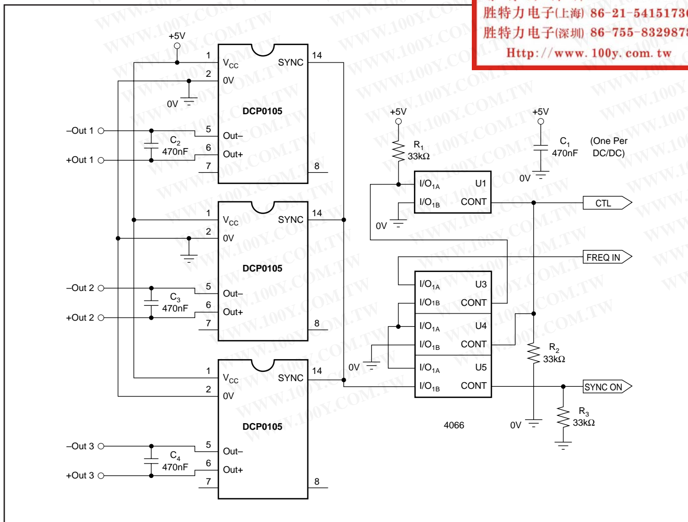
FIGURE 3. Universal Interface.
