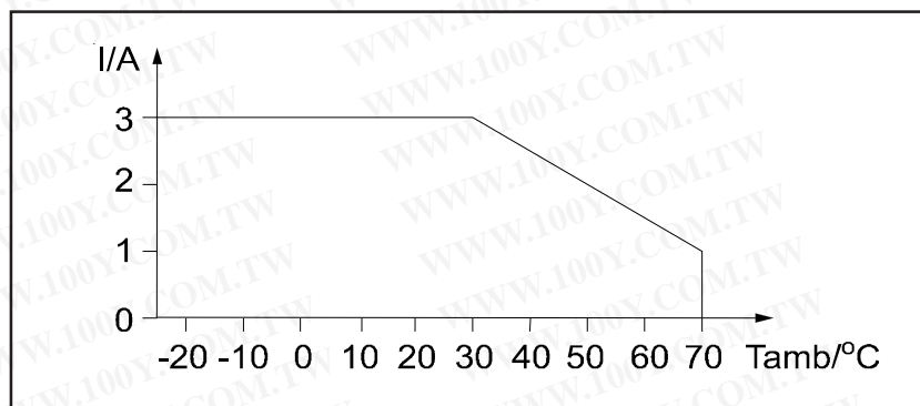
Derating curve for the relay.
