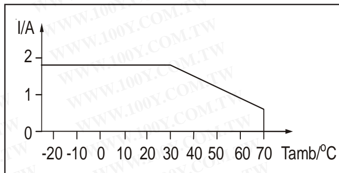
Derating curve for the relay.
