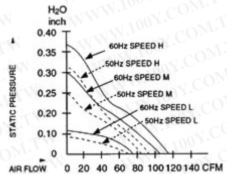
Fan Performance Curve
