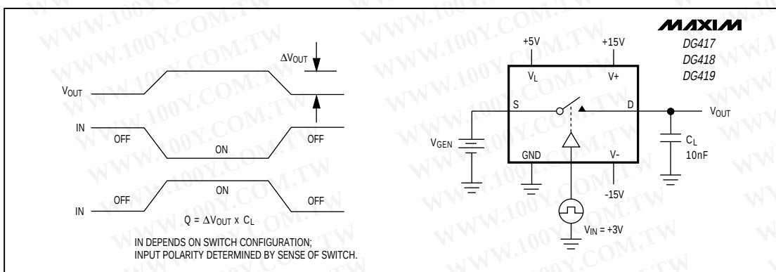
Figure 5. Charge Injection
