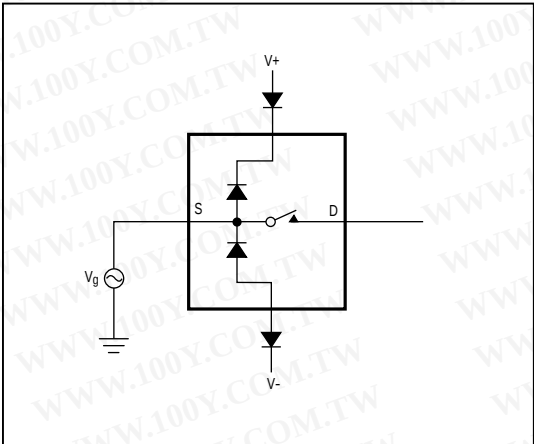
Figure 1. Overvoltage Protection Using External Blocking Diodes.
