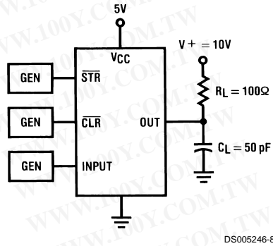
FIGURE 2. DP8311
