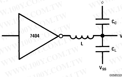
FIGURE 5. Clock Coupling
