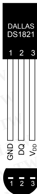
(BOTTOM VIEW)
