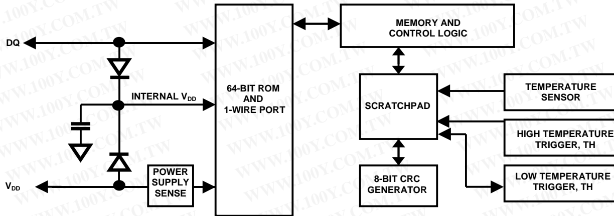
DS18S20 BLOCK DIAGRAM Figure 1
