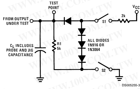
Propagation Delay (Notes 7, 9)
