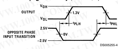
Propagation Delay (Notes 7, 9)
