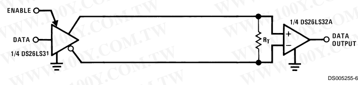
Two-Wire Balanced Interface—RS-422
