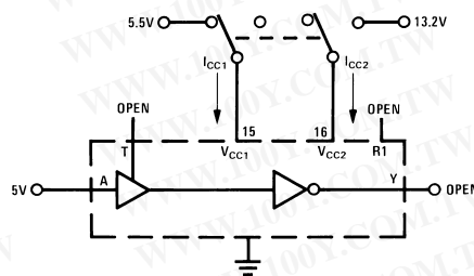
FIGURE 5. I_{CC}
