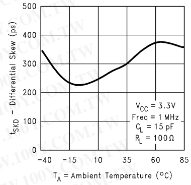
Differential Skew vs Ambient Temperature
