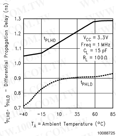
Differential Propagation Delay vs Ambient Temperature
