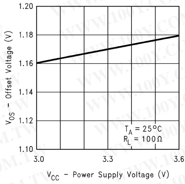
Offset Voltage vs Power Supply Voltage
