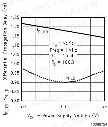
Differential Propagation Delay vs Power Supply Voltage
