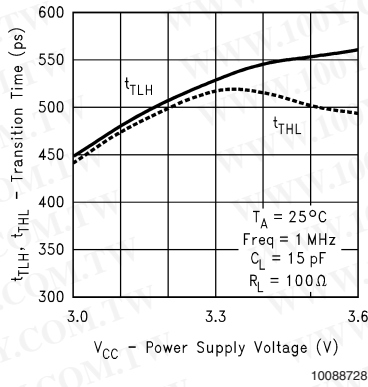
Transition Time vs Power Supply Voltage
