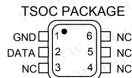
Top View 3.7 X 4.0 X 1.5 mm
