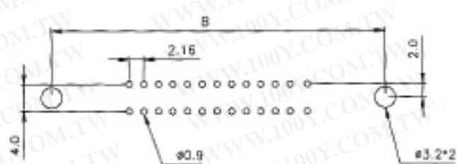
PCB LAYOUT
