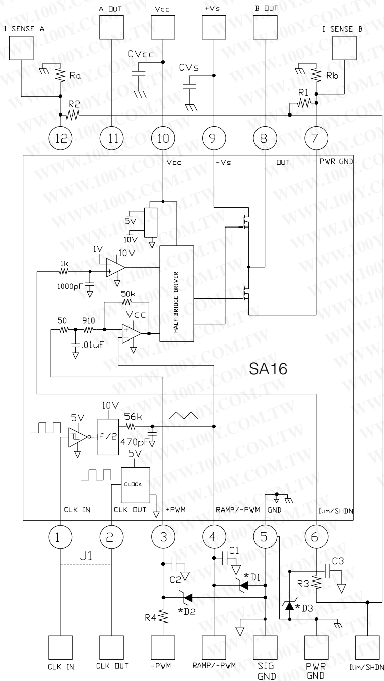
FIGURE 2. PCB SCHEMATIC.
