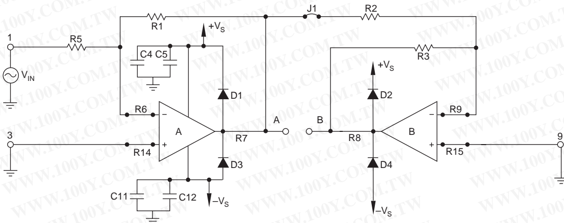
Figure 4 Dual Supply Bridge
