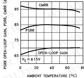
Open-Loop Gain PSRR and CMRR vs Temperature
