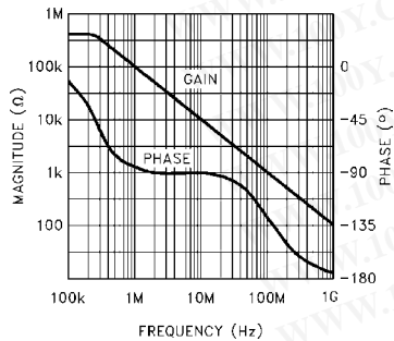
Transimpedance ( R_{oL} ) vs Frequency
