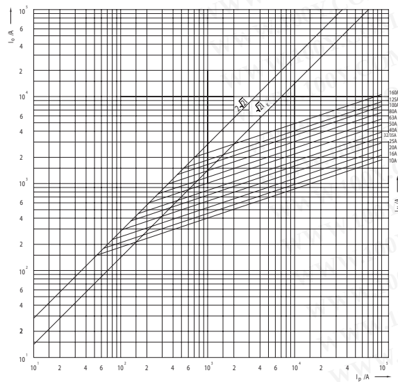
Cut-off characteristics of fuse-links Ultra Quick MUQ2, SUQ2 - size 00C
