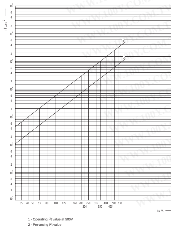
Joule Integral ( I^2t ) for Ultra Quick MUQ2, SUQ2 - size 1, 2, 3
