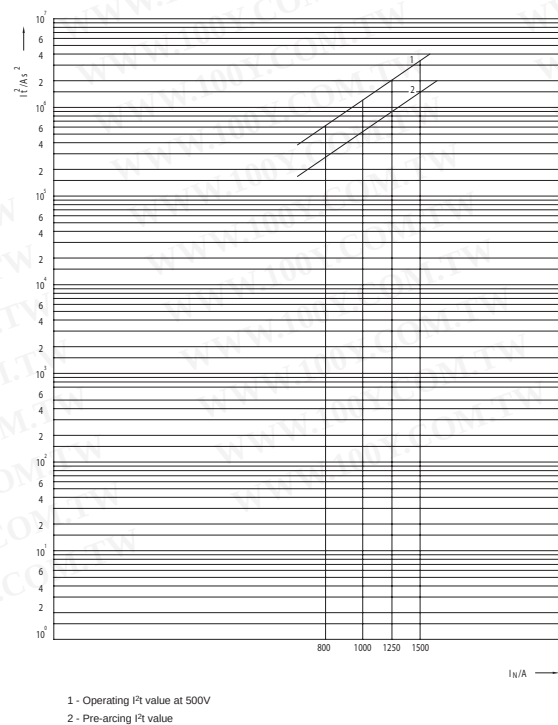
Joule Integral ( I^2t ) for Ultra Quick MUQ2, SUQ2 - size 4 and 4a
