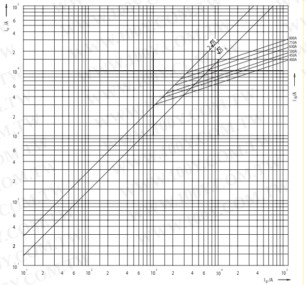
Cut-off characteristics of fuse-links Ultra Quick SUQ01, GUQ01 - size 2
