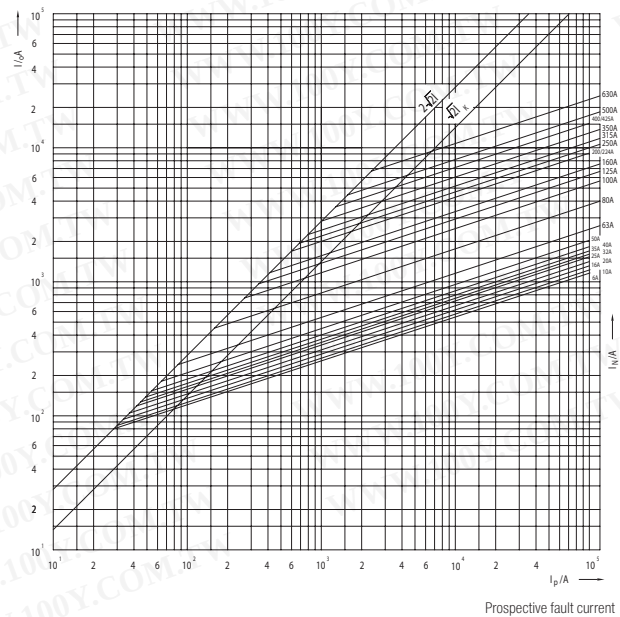
Cut-off characteristics of fuse-links Ultra Quick MUQ2, SUQ2, GUQ2 - size 00C, 1, 2, 3
