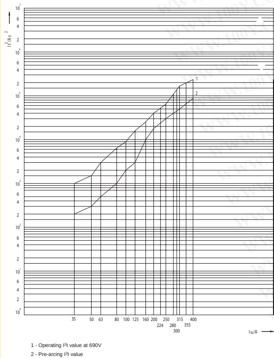
Joule Integral ( I^2t ) for Ultra Quick MUQ U-N, SUQ U - size 1, 2
