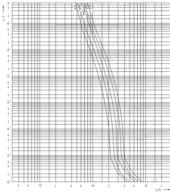
Time/current characteristics of fuse-links Ultra Quick SUQ1, GUQ1 - size 2
