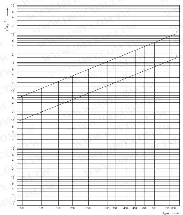
Joule Integral ( I^2t ) for Ultra Quick SUQ1, GUQ1 - size 1, 2, 3
