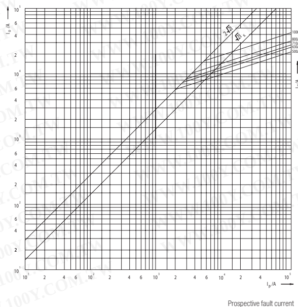
Cut-off characteristics of fuse-links Ultra Quick SUQ01, GUQ01 - size 3
