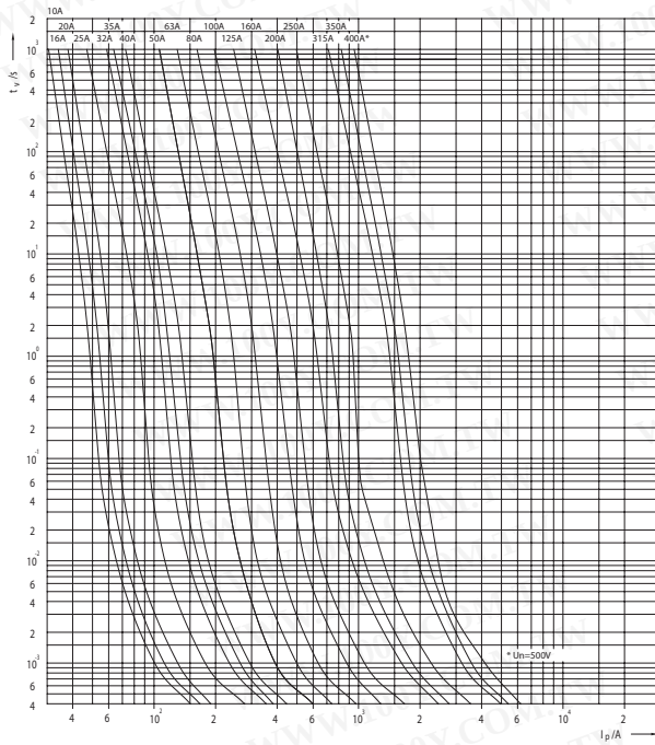
Time/current characteristics of fuse-links Ultra Quick MUQ1, SUQ1 - size 00C and 00
