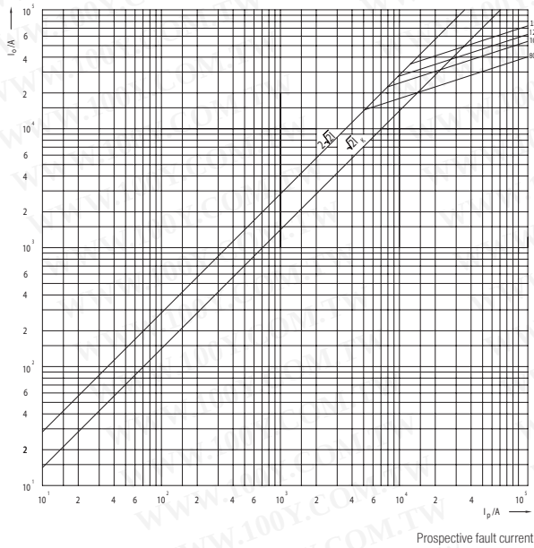
Cut-off characteristics of fuse-links Ultra Quick MUQ2, SUQ2 - size 4 and 4a
