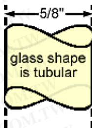
usual shape of T-5 glass envelopes (not to scale)
