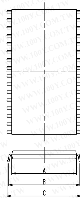
FP-32-1.27 (REFERENCE ONLY)
