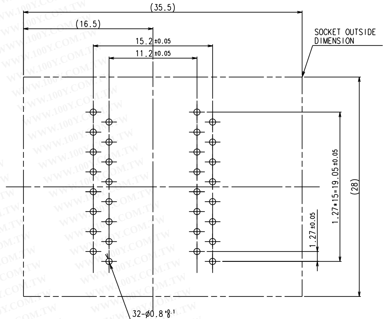
FP-32-1.27 (REFERENCE ONLY)
