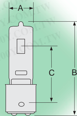
BA15d
