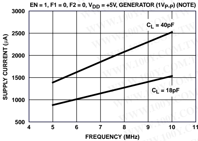
FIGURE 19. SUPPLY CURRENT vs FREQUENCY
