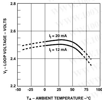
Figure 5. Typical Input Voltage vs. Temperature.
