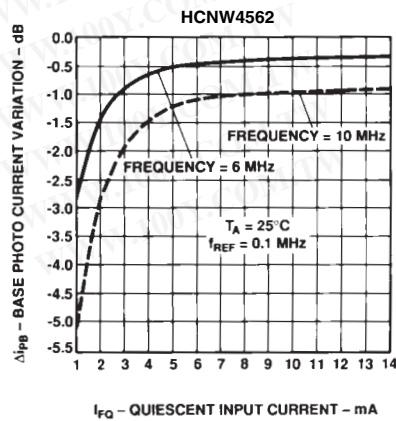
Figure 10. Base Photo Current Variation vs. Bias Conditions.
