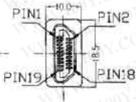
HDMI 19P FEMALE
