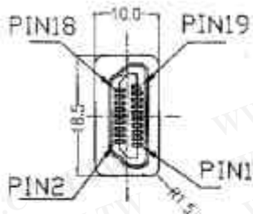
HDMI 19P FEMALE
