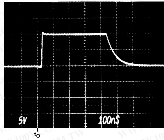
FIGURE 2B. V_{IN} = +10V
