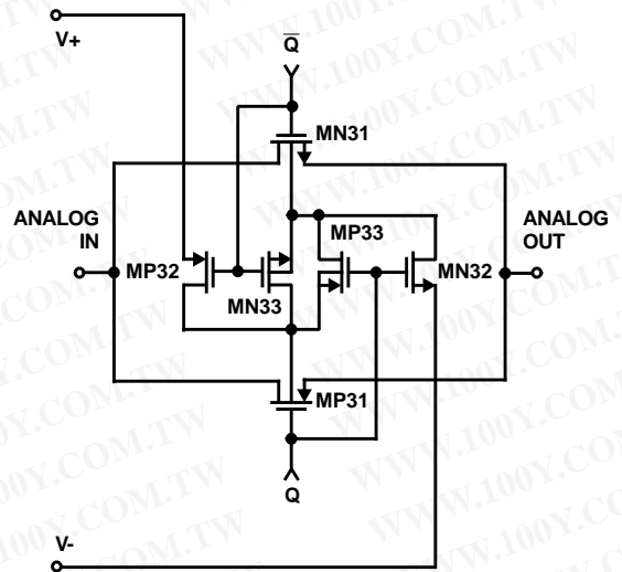
SWITCH CELL
