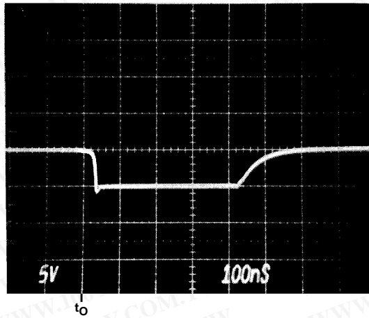
FIGURE 2E. V_{IN} = -5V
