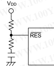
Reset circuit
