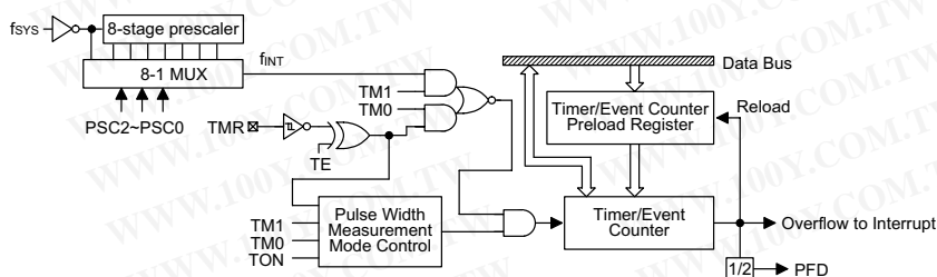
Timer/Event Counter
