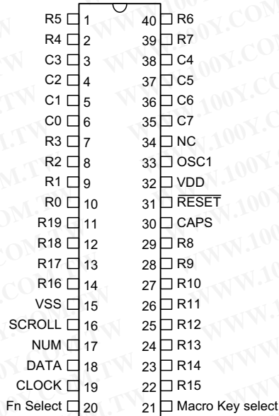
HT82K628A - 40 DIP
