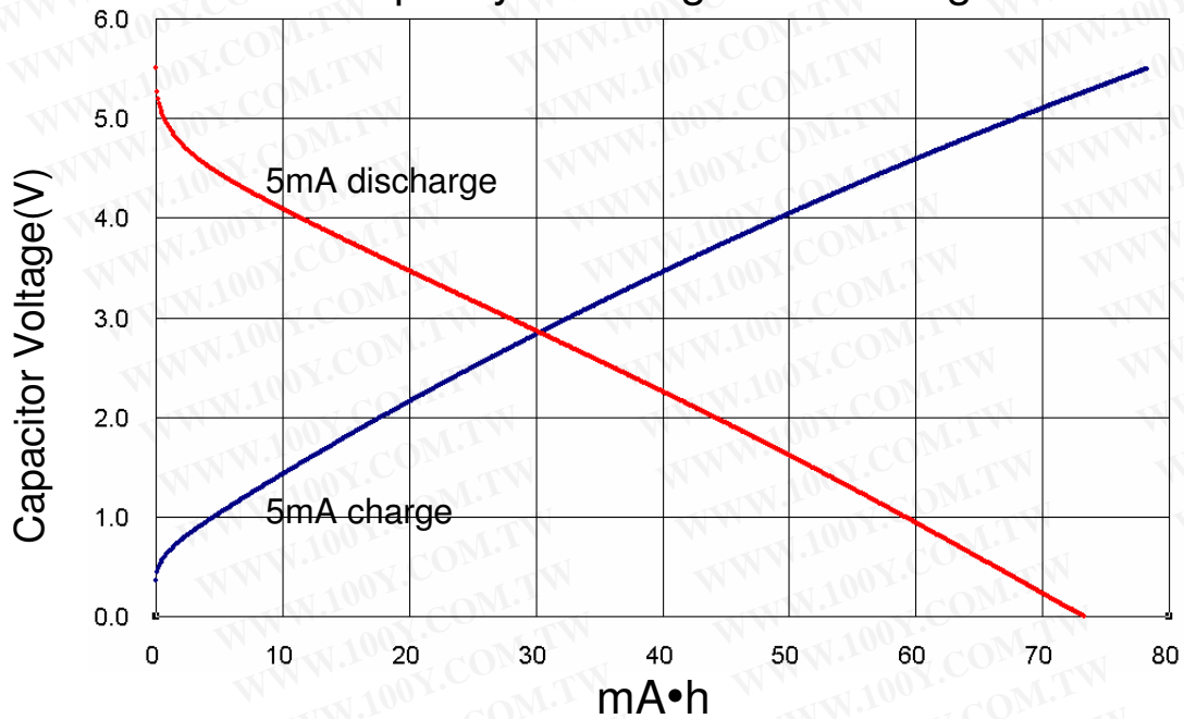
Capacity of Charge & Discharge
