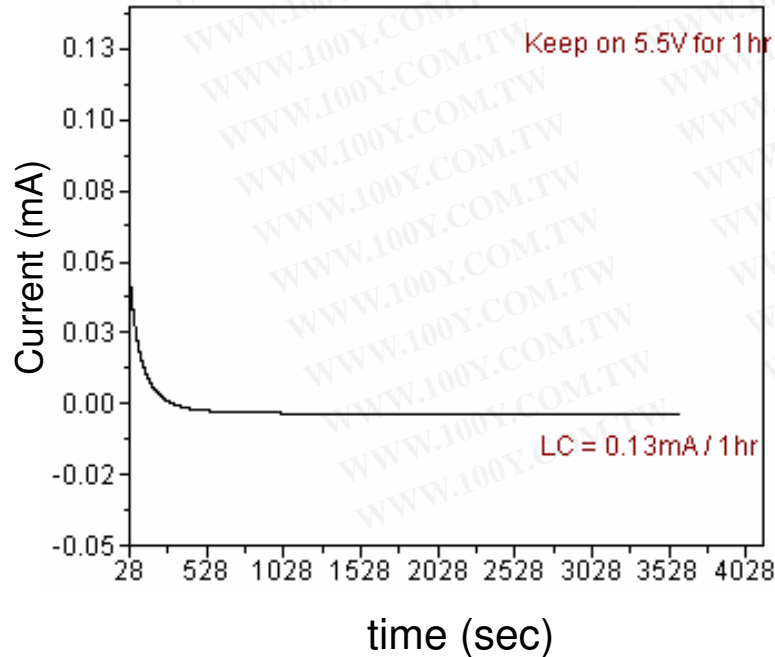
Leakage Current Test
