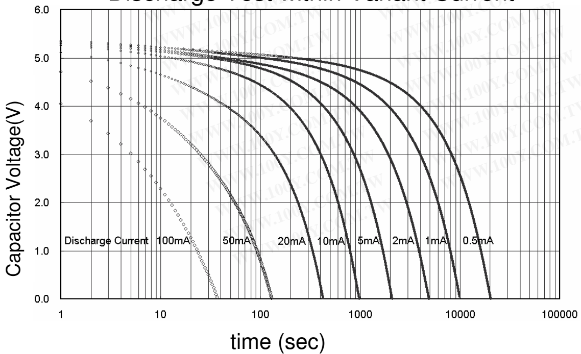
Discharge Test within Variant Current
