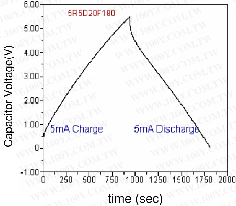
Charge – Discharge Curve
