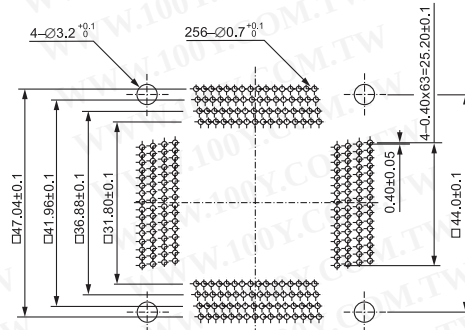
IC51-2564-1668 (256 Pins)
