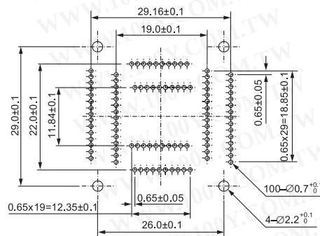
IC51-814-KS12033 (100 Pins)
