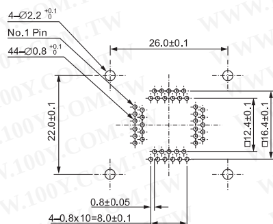
IC51-0444-798 (44 Pins)
