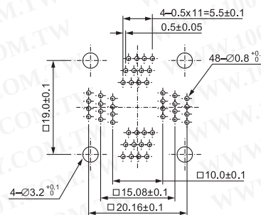
IC51-0484-806 (48 Pins)
