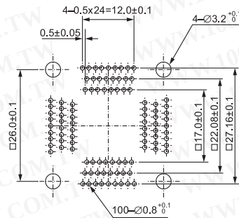
IC51-1004-809 (100 Pins)
