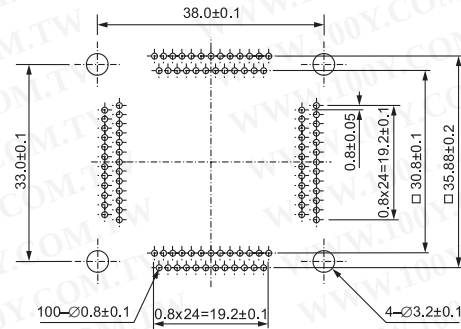
IC51-1124-1036-2 (112 Pins)
