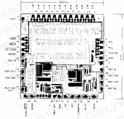
Chip Topography
