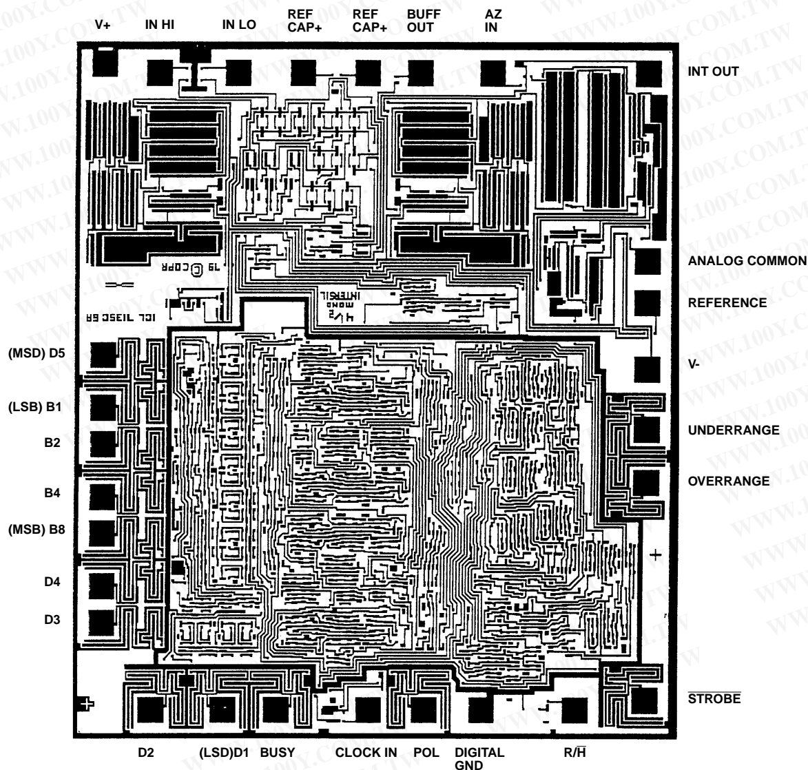
ICL7135
