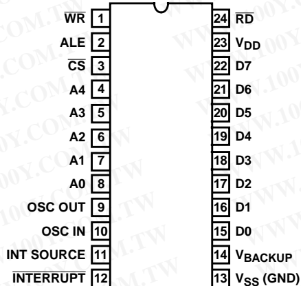
ICM7170 (PDIP, SBDIP) TOP VIEW
