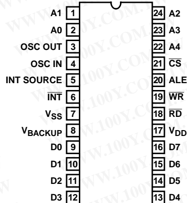
ICM7170 (SOIC) TOP VIEW
