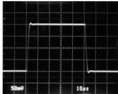
SMALL-SIGNAL STEP RESPONSE C_L = 200\text{pF}
