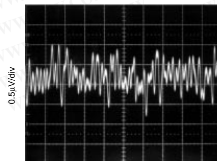
0.1 to 10Hz PEAK-TO-PEAK VOLTAGE NOISE
